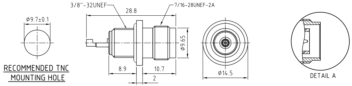
RP TNC DETAIL DRAWING
